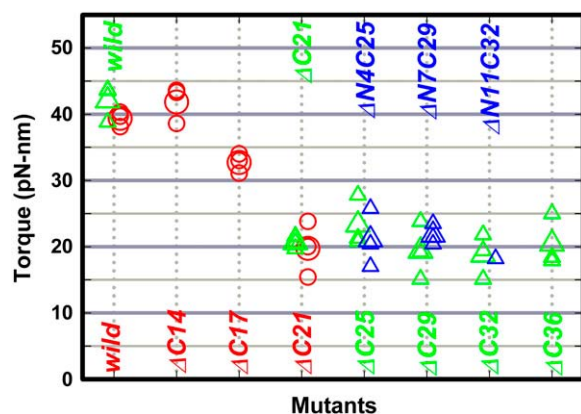
FIGURE 6 Torque of gamma deletion mutants. Green, this study; red (26) and blue (27), previous results. Circles, torque estimated with a duplex of 0.49- \mu m beads; triangles, 0.29- \mu m bead duplex. Small symbols represent individual estimations, and large symbols represent their average.
