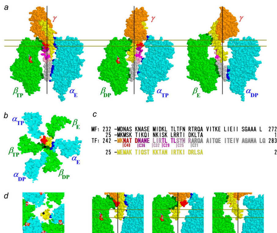
FIGURE 1 Atomic structure of MF 1 (22). Truncations of γ-subunit are shown, with color scheme in c; the N-terminal α-helix is shown in yellow. Those atoms of α-subunits and β-subunits that are within 0.5 nm from an atom of γ (excluding hydrogens) are colored blue and dark green, respectively. Nucleotides are shown in CPK colors. Black lines in side views and black dots in bottom views represent putative rotation axis (21). (a) Side views show central γ and an opposing α-β pair. Membrane-embedded F 0 portion of ATP synthase would be above the γ-subunit. (b) Bottom view of section between pair of gold lines in a. (c) Amino-acid sequences at the C-terminus and N-terminus of γ in MF 1 (36) and TF 1 (30), except that numbering for TF 1 in our study here starts from Met-1, which is absent in the expressed wild-type protein. In Fig. 1 B of Furuike et al. (27), Ala-2 was incorrectly shown as Ala-1. (d) Central portions of bottom and side views for γ-ΔC36.
